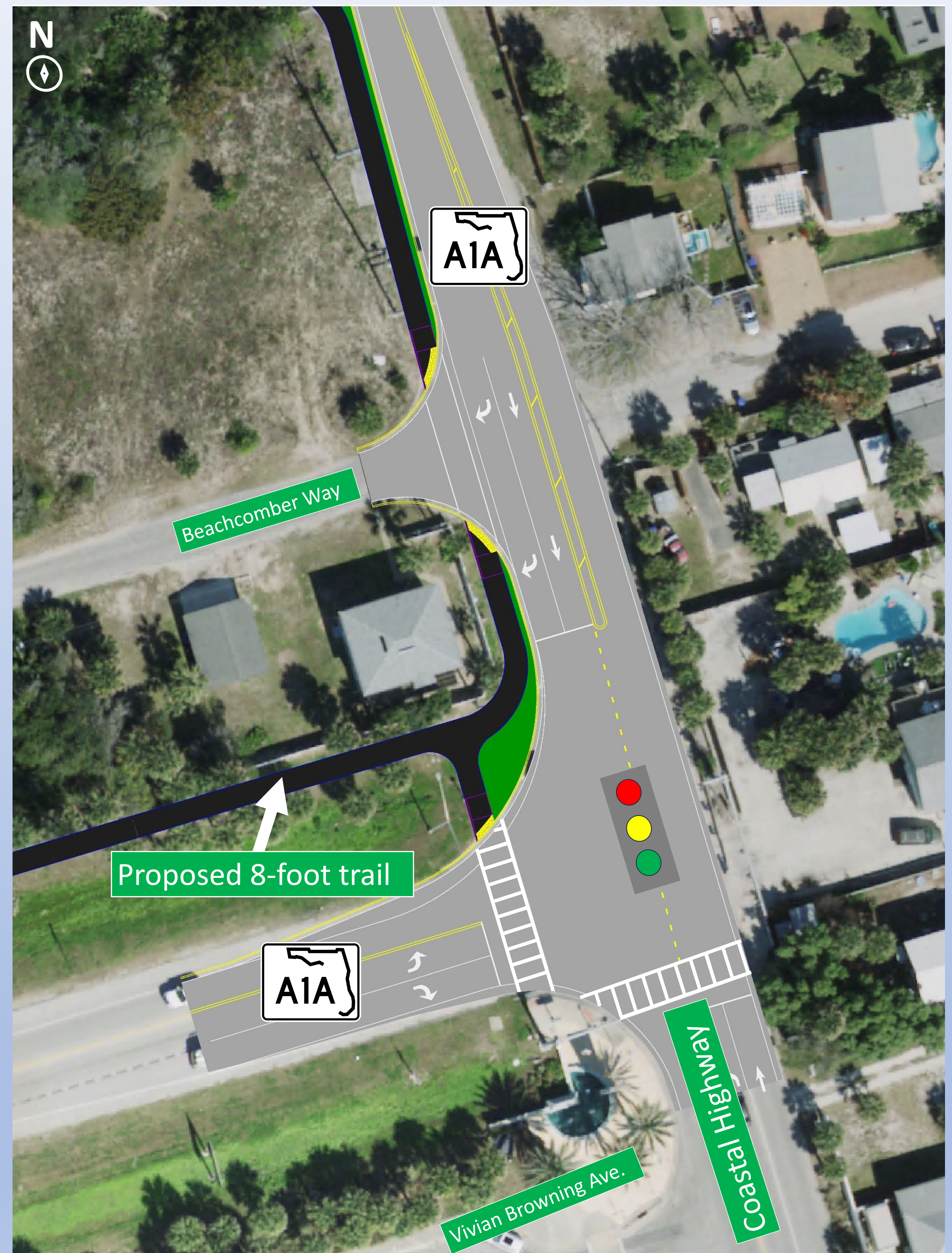
PROPOSED INTERSECTION IMPROVEMENTS AND TRAIL
